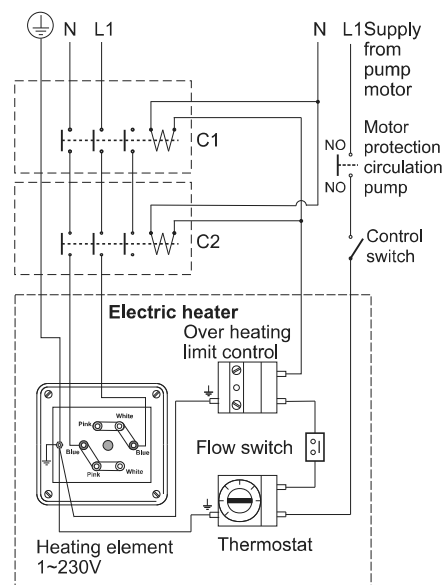
1-phase 230V
