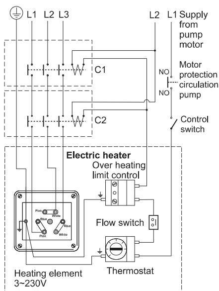
3-phase 230V
