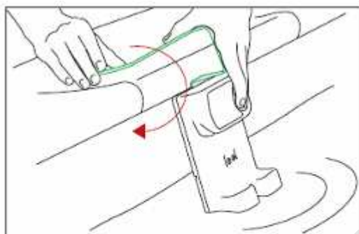
Sensor Espio™ must be fully flat against the wall. Adjust the attachment support if need be. If there is a gap between the attachment support and the coping, put the wedging foam pad in it (cut it down to size if need be).
